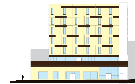
East Elevation 1"=1/16"
