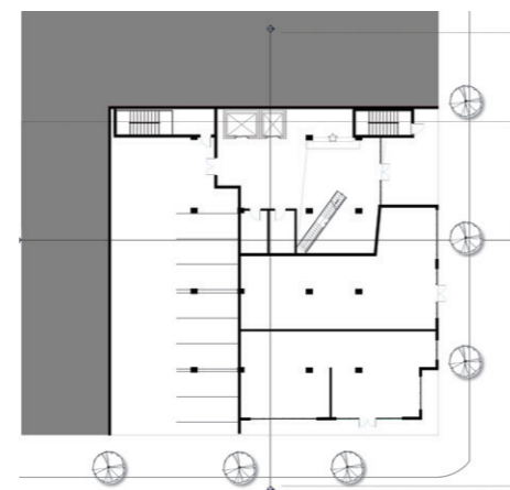
1st Floor Plan 1"=1/16" N
