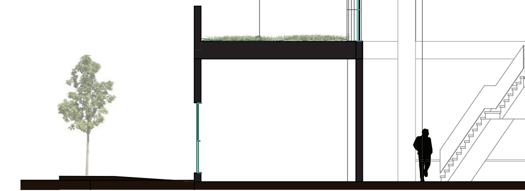
Wall Section 1"=3/8"
