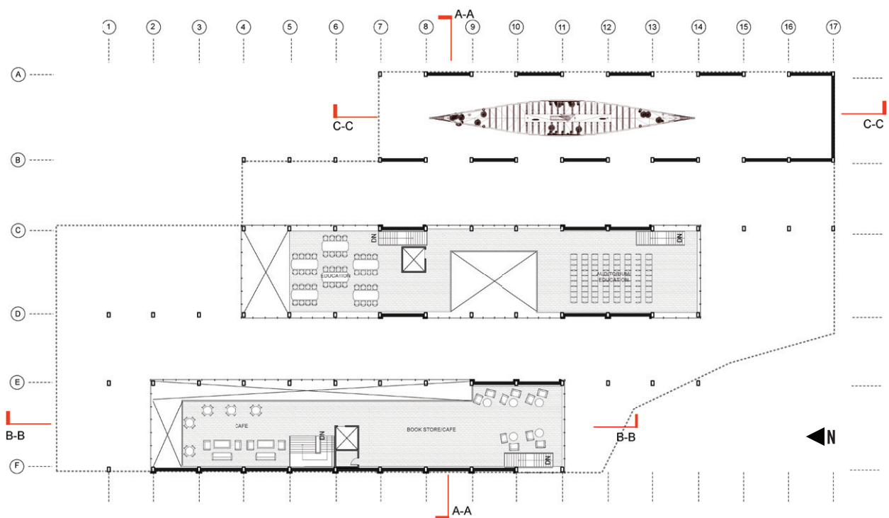
PLAN FIRST FLOOR
