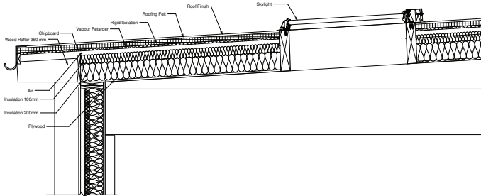
SECTION F-F
