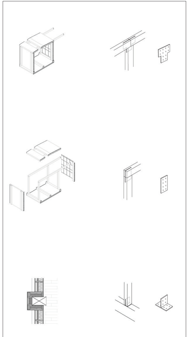
SCALE 1:20
